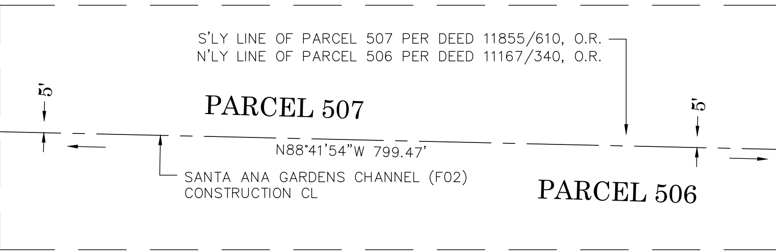
DETAIL C SCALE: 1"=40'
