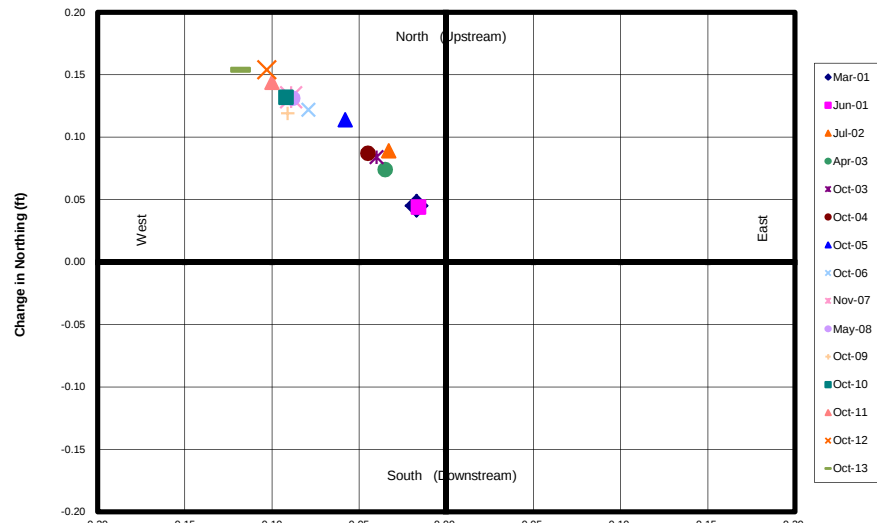
Inclinometer Monitoring Point SI-5
