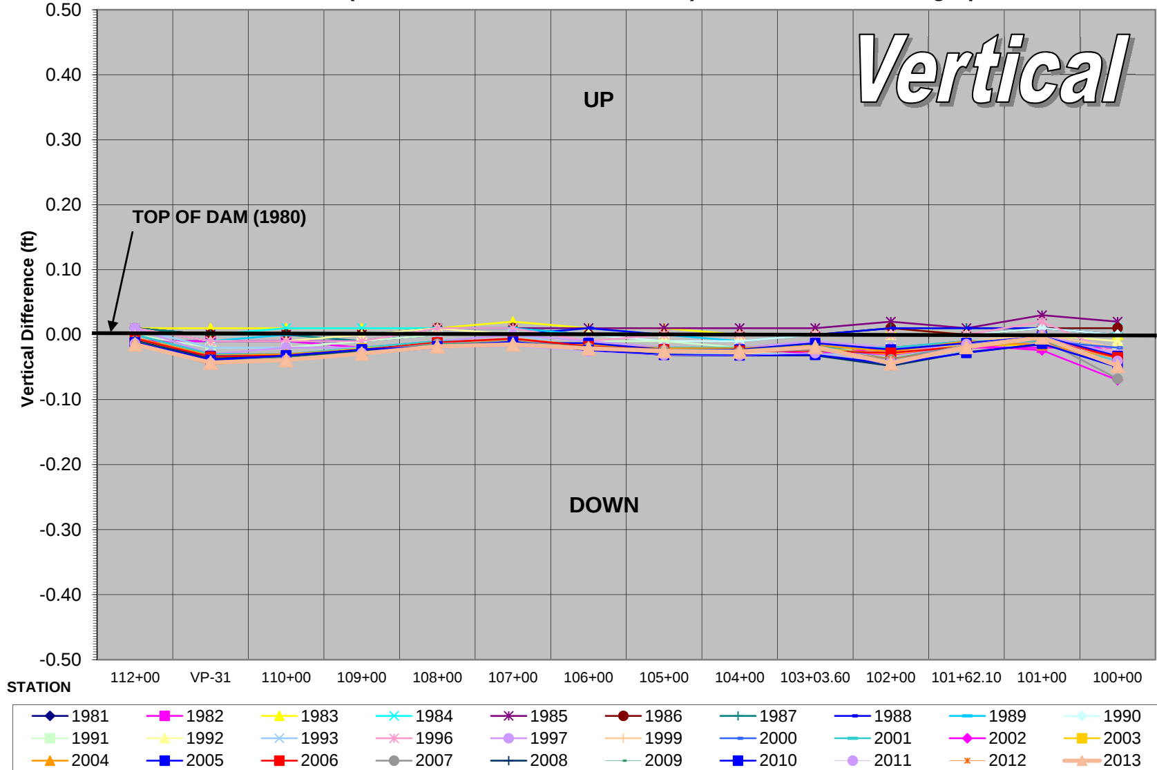
Vertical Movement (Difference from 1980 Elevations) - Profile View - Looking Upstream
