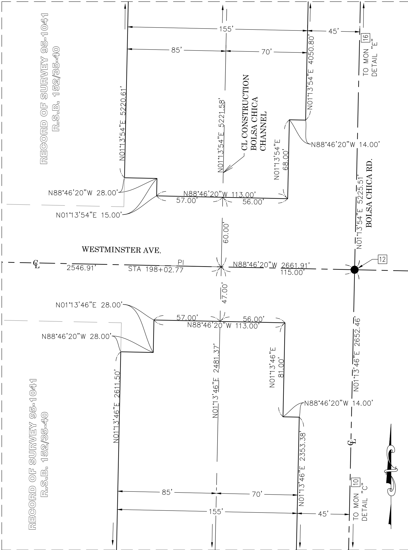
DETAIL "D" SCALE:1"=40'
