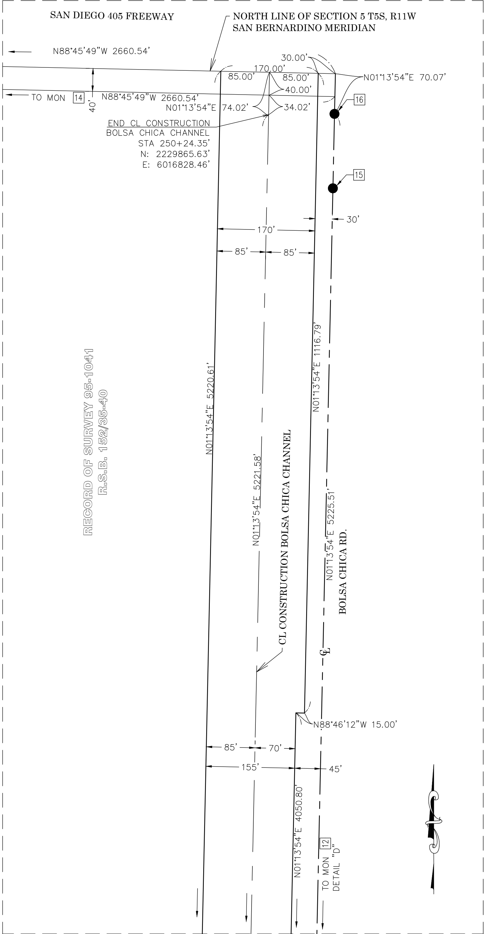
DETAIL "E" SCALE:1"=100'
