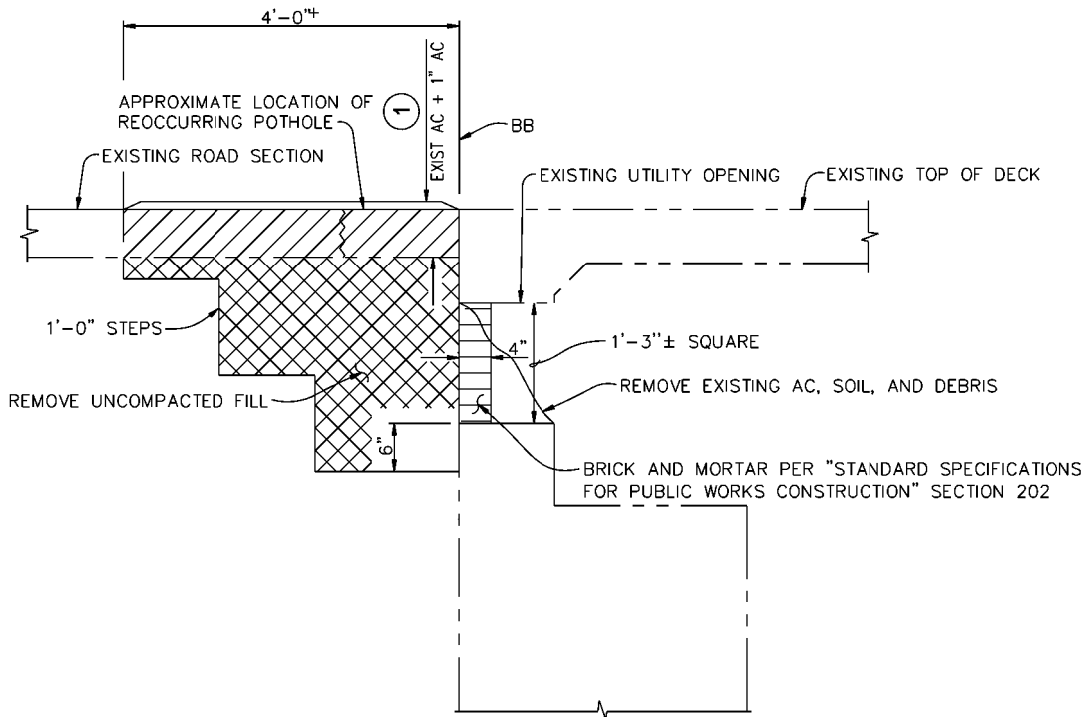
A NORTH ABUTMENT NOT TO SCALE
