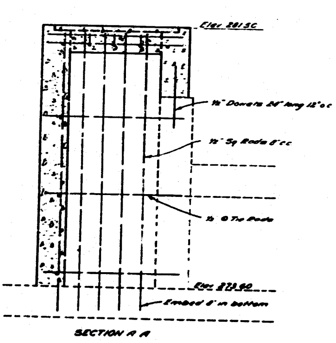
DETAIL OF CATCH BASIN STA 66+07.8 Scale 1"=2'
