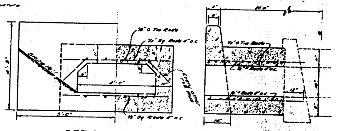
DETAIL OF CULVERT EXTENSION STA 232+36 Both Ends To Be Extended Scale 1"=2'
