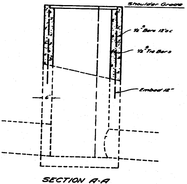
DETAIL OF CATCH BASIN STA 66+07.8 Scale 1"=2'
