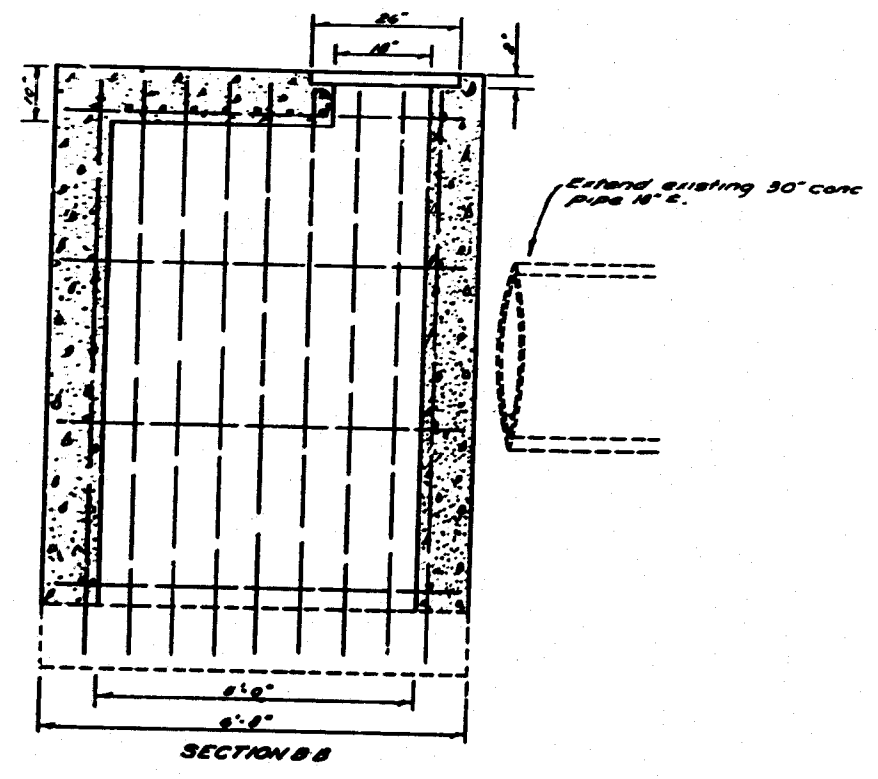
DETAIL OF CATCH BASIN STA 66+07.8 Scale 1"=2'
