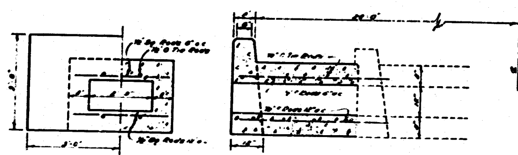
DETAIL OF CULVERT EXTENSION STA 138+53 Both Ends To Be Extended Scale 1"=2'
