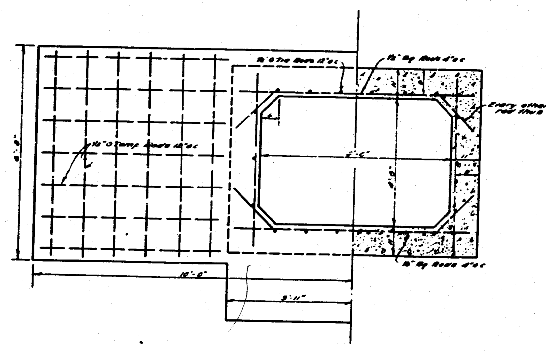
DETAIL OF CULVERT EXTENSION STA 166+39 Both Ends To Be Extended Scale 1"=2'
