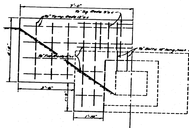
DETAIL OF HEADWALL CONSTRUCTION STA 34+56 Construct South Headwall As Shown Scale 1"=2'
