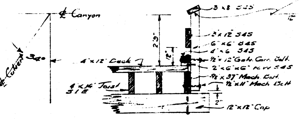
HANDRAIL DETAIL Scale "2"=1'
