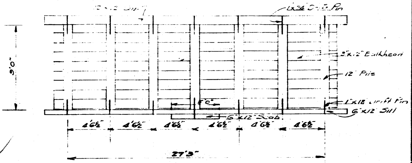
BULKHEAD ELEVATION Scale 1/4"=10'
