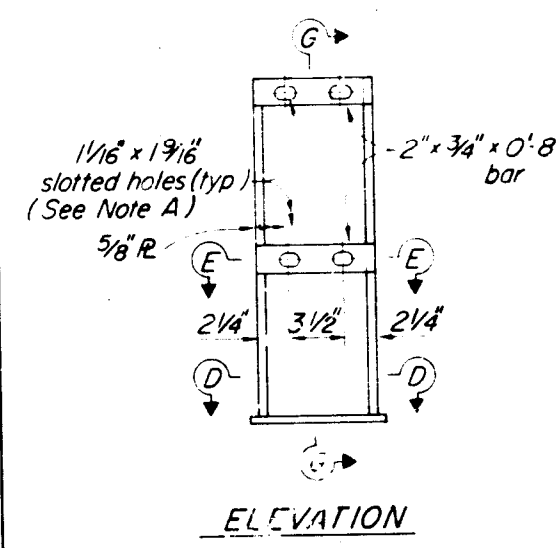
POST SHIM DETAIL TYPES 9 & 11
