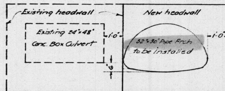
ELEVATION OF NORTH EAST HEADWALL
