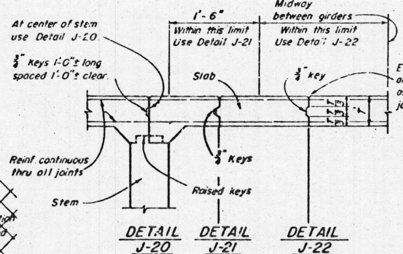
PART SECTION INTERIOR GIRDER
