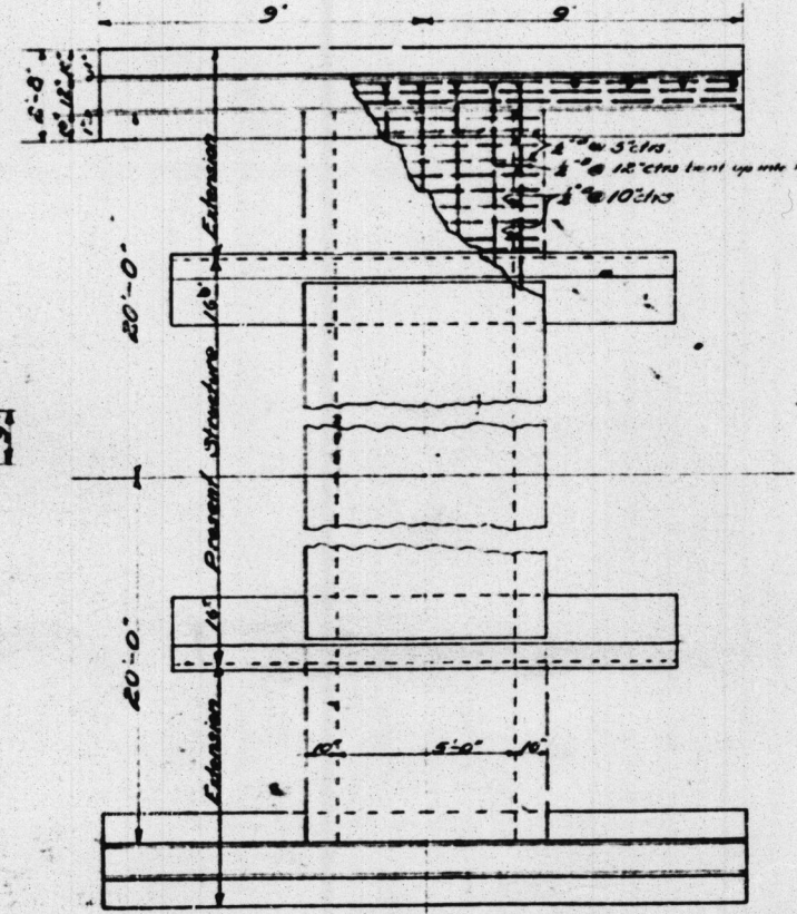
DETAILS OF 5x3 BOX CULVERT Sta. 208+57 Both Ends to be Extended
