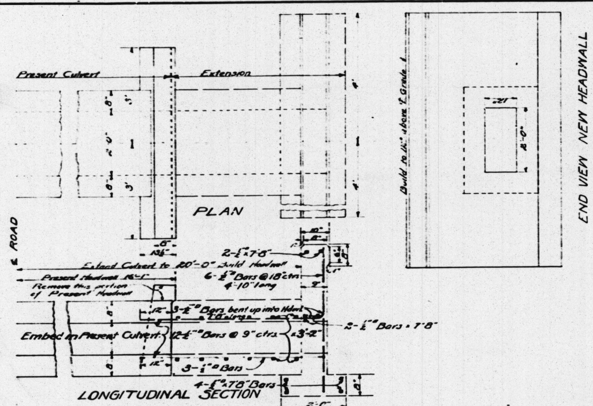
DETAIL OF CULVERT EXTENSION Sta. 177+36 South End Only to be Extended Scale: 1/2" = 1'
