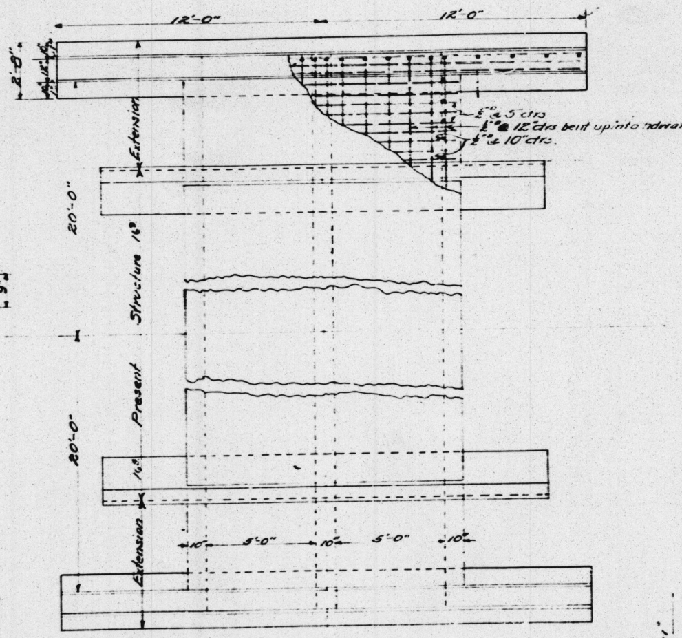
DETAILS OF DOUBLE 5x3 BOX CULVERT Sta. 205+36 Both Ends to be Extended to 20' From &
