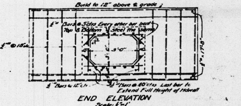
DETAILS OF 5x3 BOX CULVERT Sta. 208+57 Both Ends to be Extended
