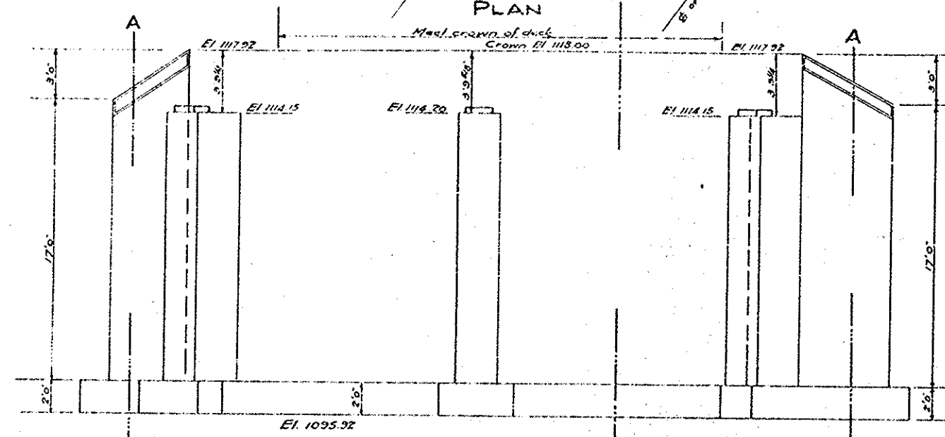
DETAILS OF NORTH ABUTMENT Scale 3/8"=1'-0"
