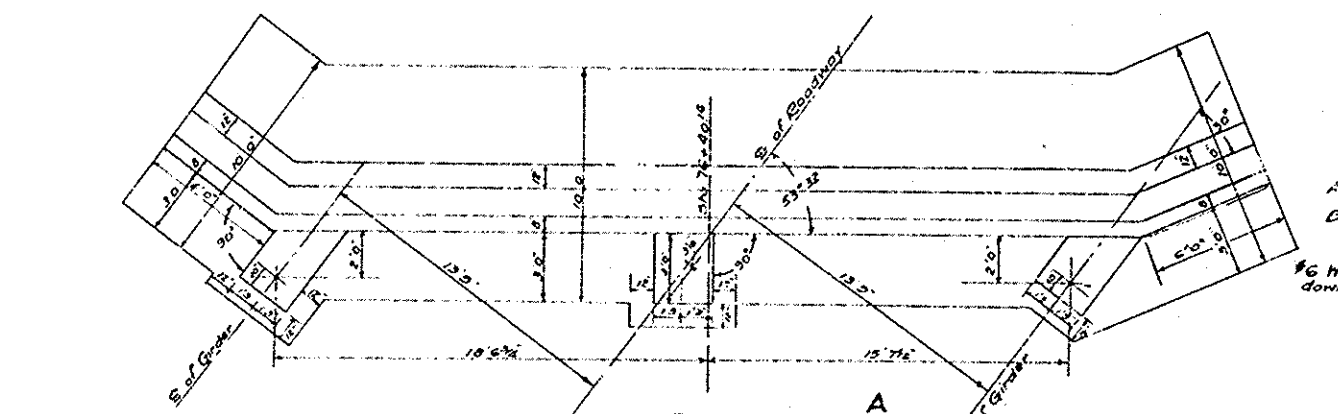
SECTION H-H Scale 3/8"=1'-0"
