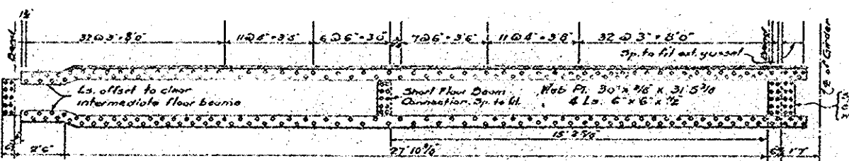
SECTION ALONG NEW END FLOOR BEAM
