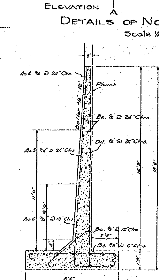
SECTION B-B Scale 3/8"=1'-0"
