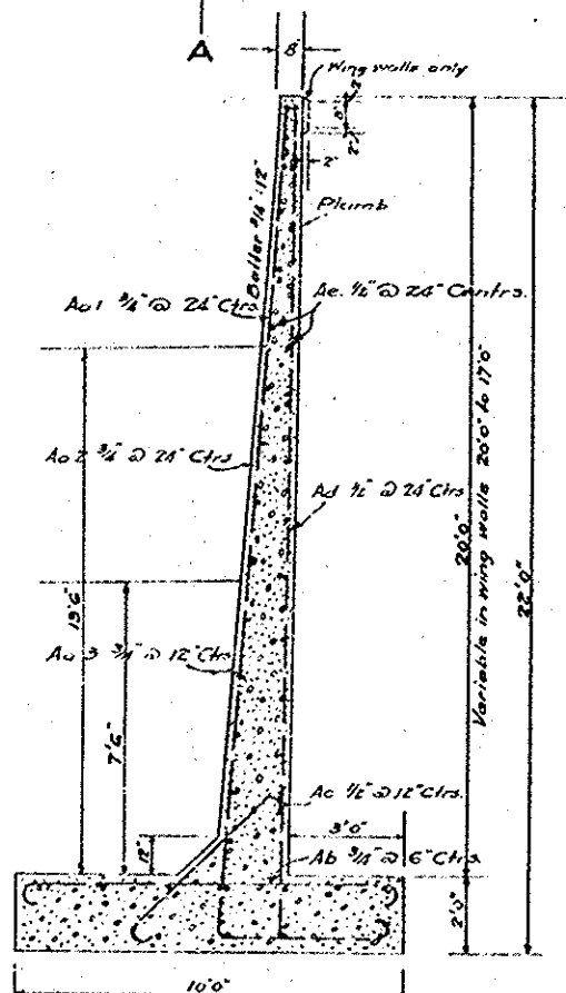
SECTION A-A Scale 3/8"=1'-0"
