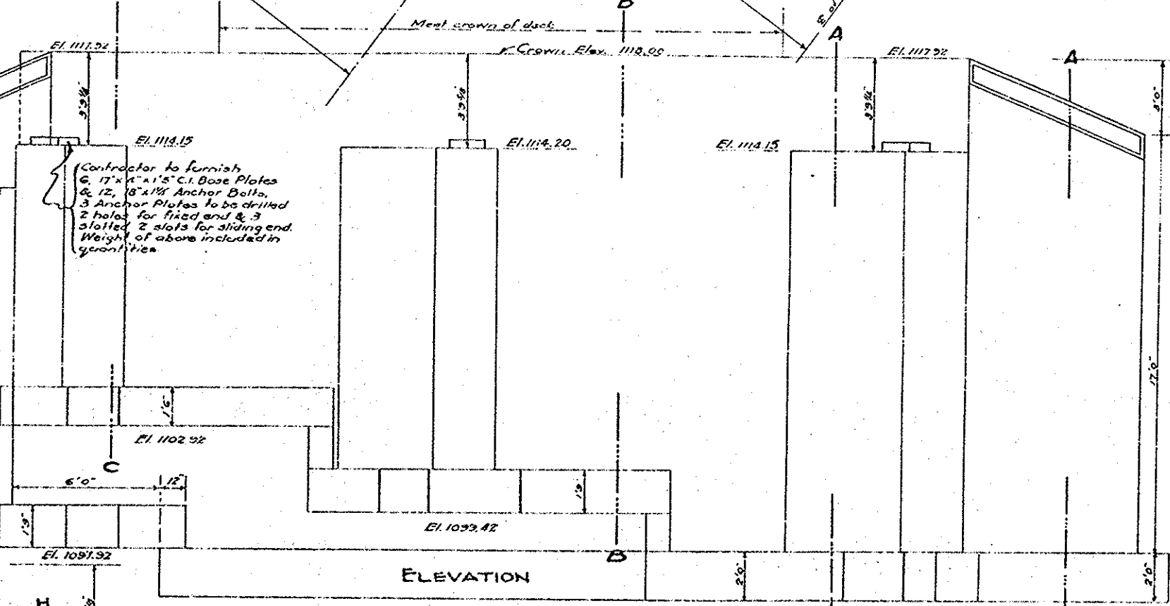
DETAILS OF SOUTH ABUTMENT Scale 3/8"=1'-0"
