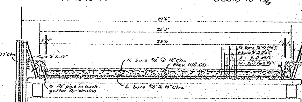
CROSS SECTION THRU DECK Scale 3/8"=1'-0"
