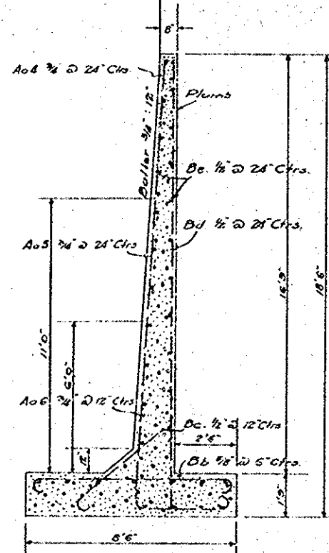
SECTION B-B Scale 3/8" = 1'-0"
