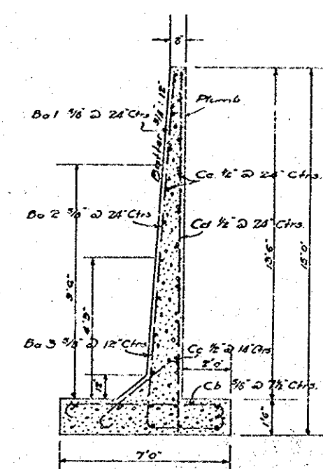
SECTION C-C Scale 3/8" = 1'-0"
