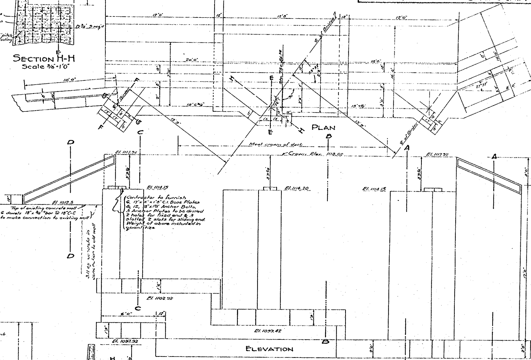
ELEVATION B DETAILS OF SOUTH ABUTMENT Scale 3/8" = 1'-0"
