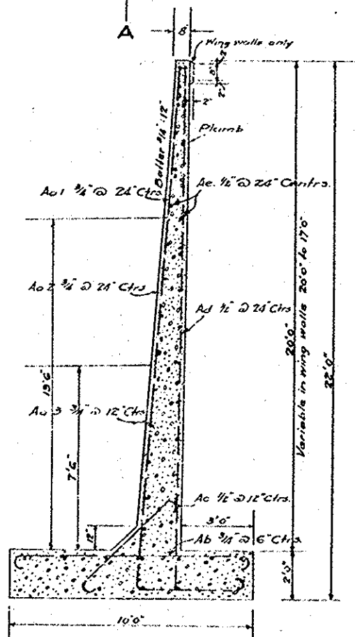
SECTION A-A Scale 3/8" = 1'-0"
