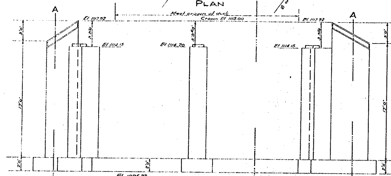
ELEVATION A DETAILS OF NORTH ABUTMENT Scale 1/2" = 1'-0"
