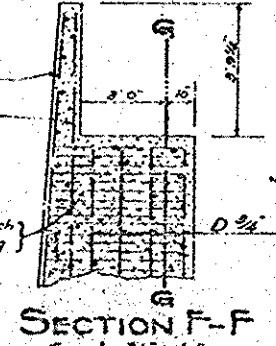
SECTION F-F Scale 3/8" = 1'-0"
