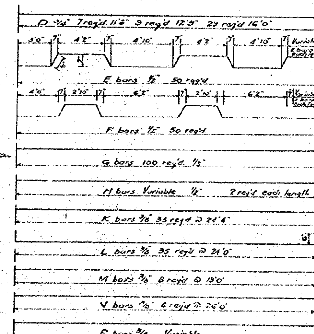
REINFORCING STEEL DETAILS NOT TO SCALE
