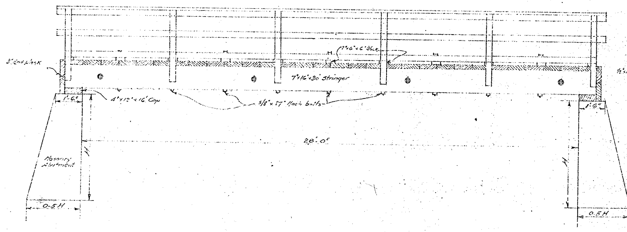
ELEVATION Scale 1/2" = 1'
