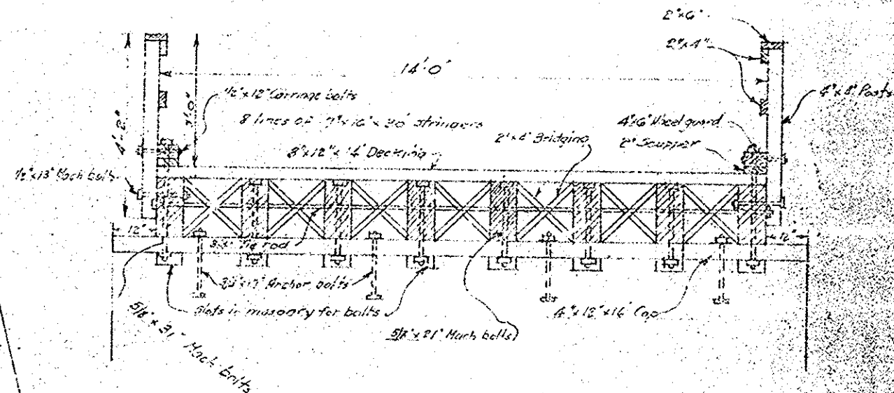
SECTION THRU BRIDGE
