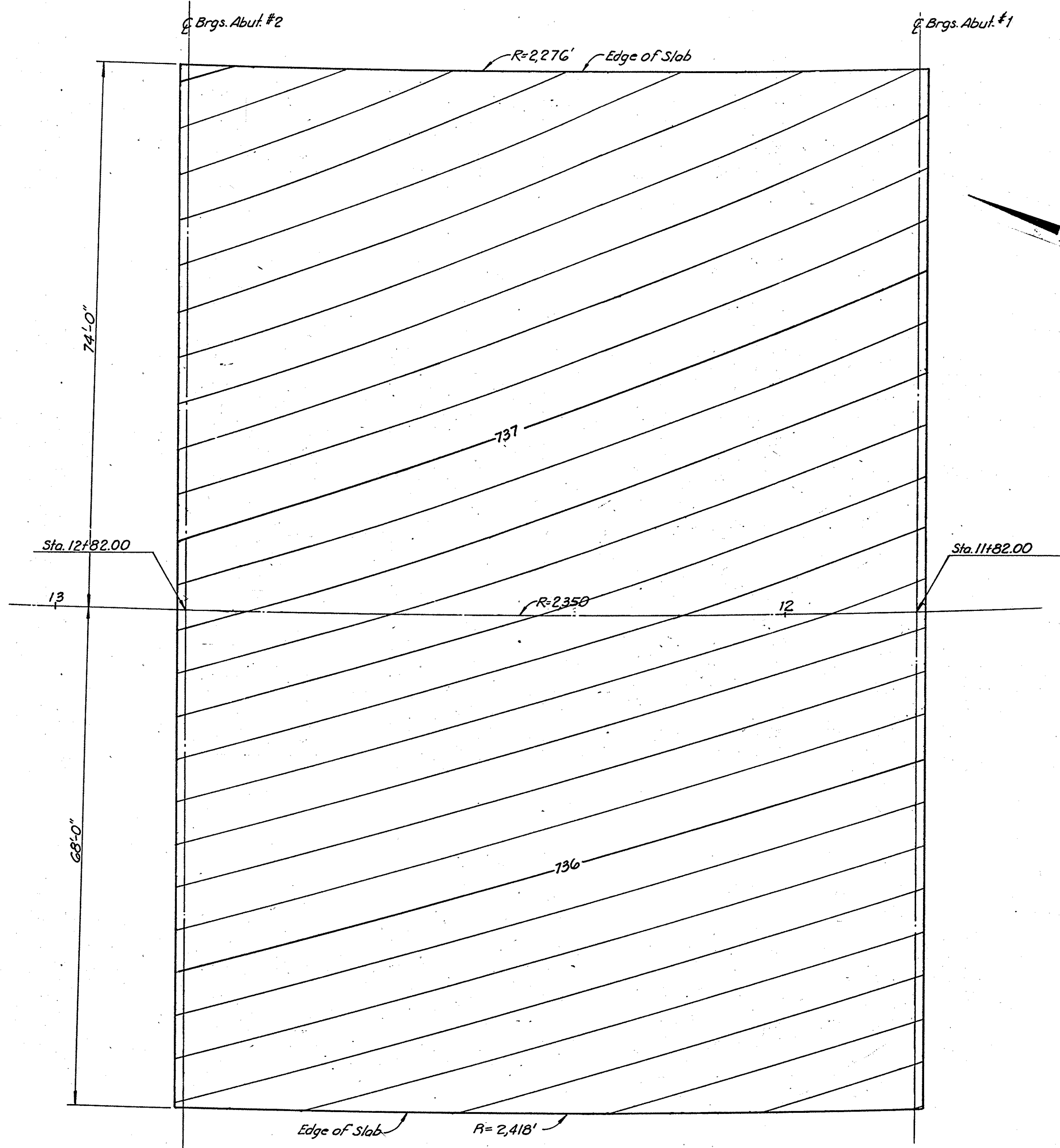
BRIDGE DECK CONTOURS Scale: 1"=10'
