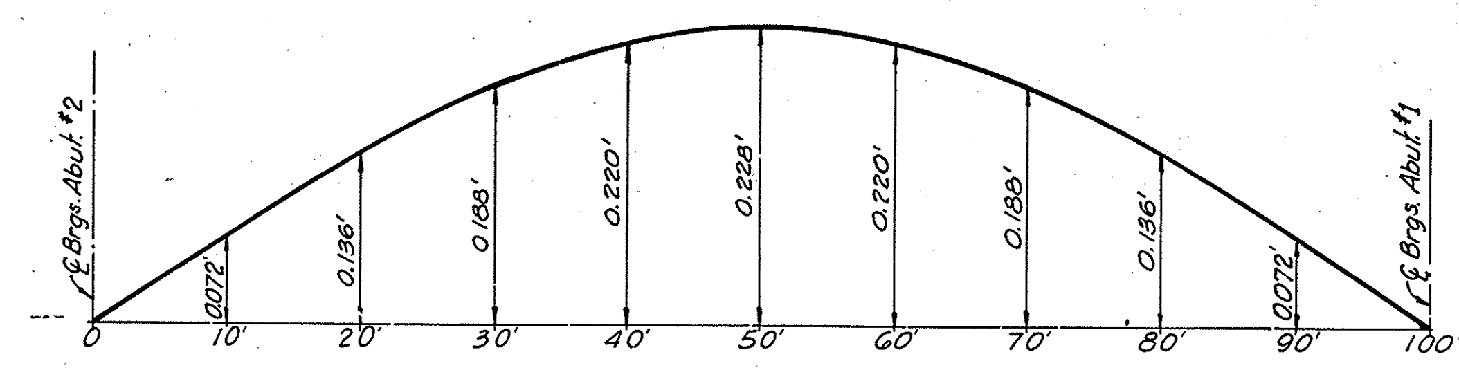
CAMBER DIAGRAM Camber diagram does not include falsework settlement or deflection.
