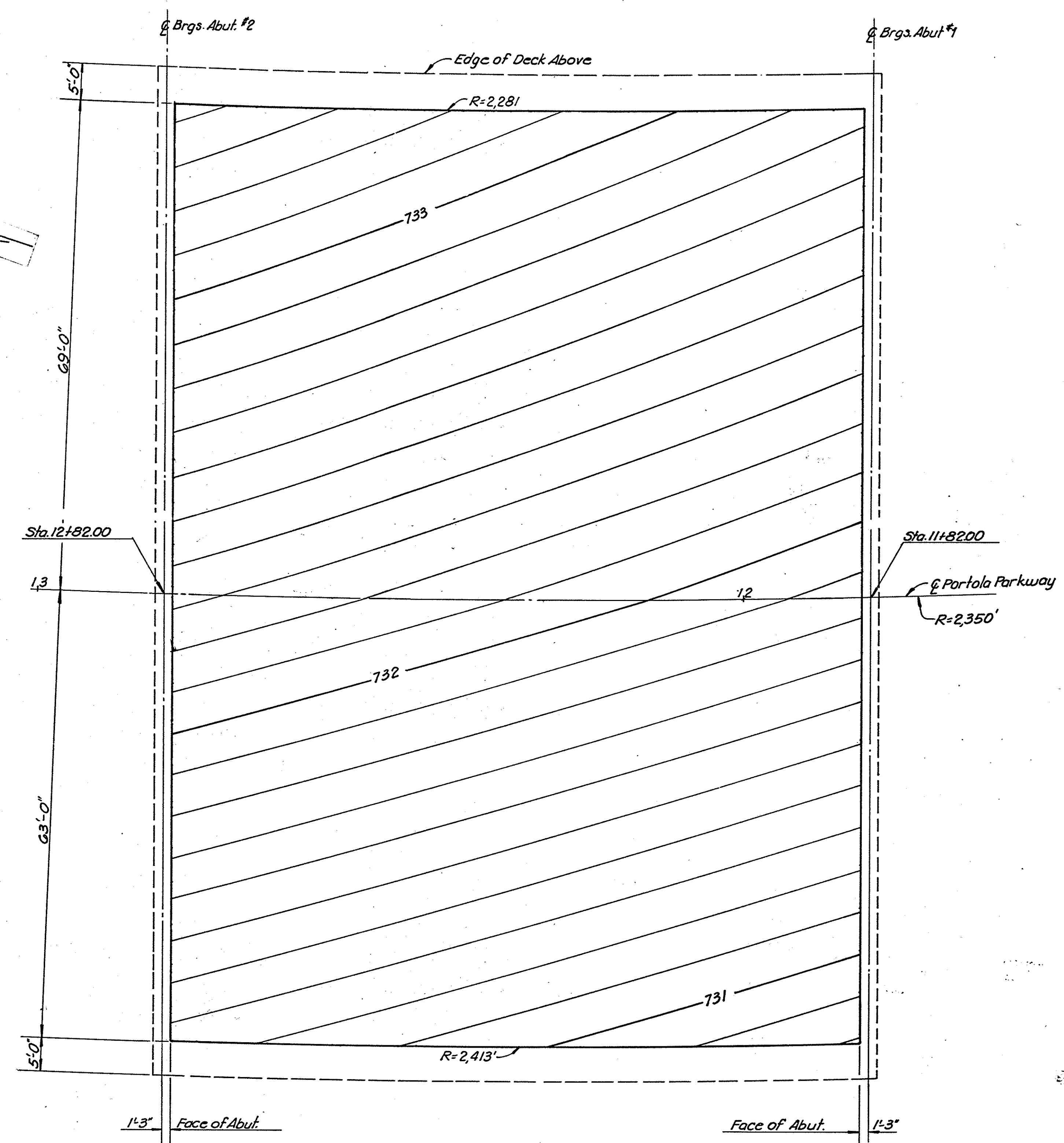
BRIDGE SOFFIT CONTOURS Scale: 1"=10'
