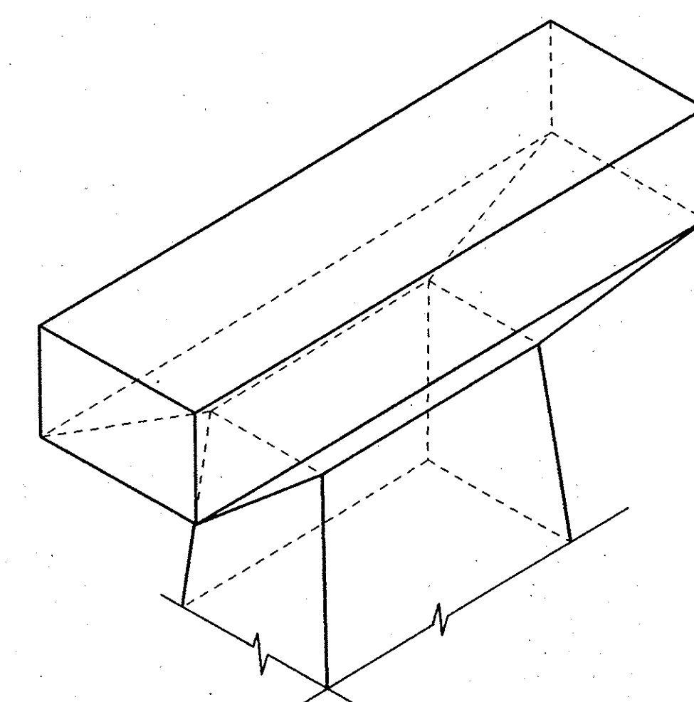
ISOMETRIC VIEW - PIER CAP
