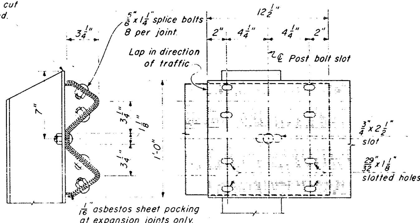
CROSS SECTION
