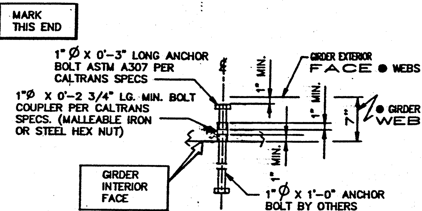
DETAIL 1 SCALE 1 1/2"=1'-0" G-3
