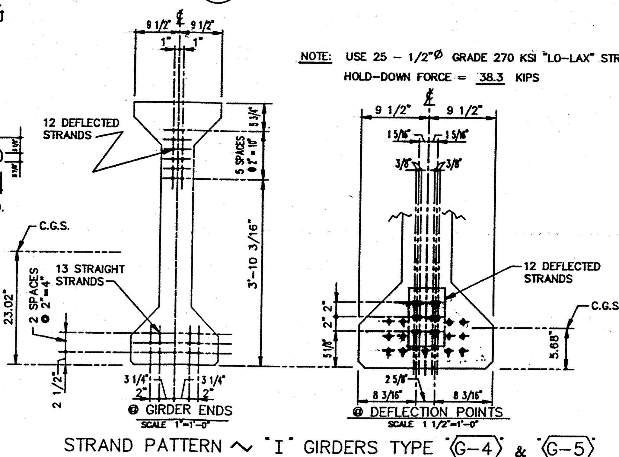
HALF GIRDER ELEVATION SCALE: 1/2" = 1'-0"
