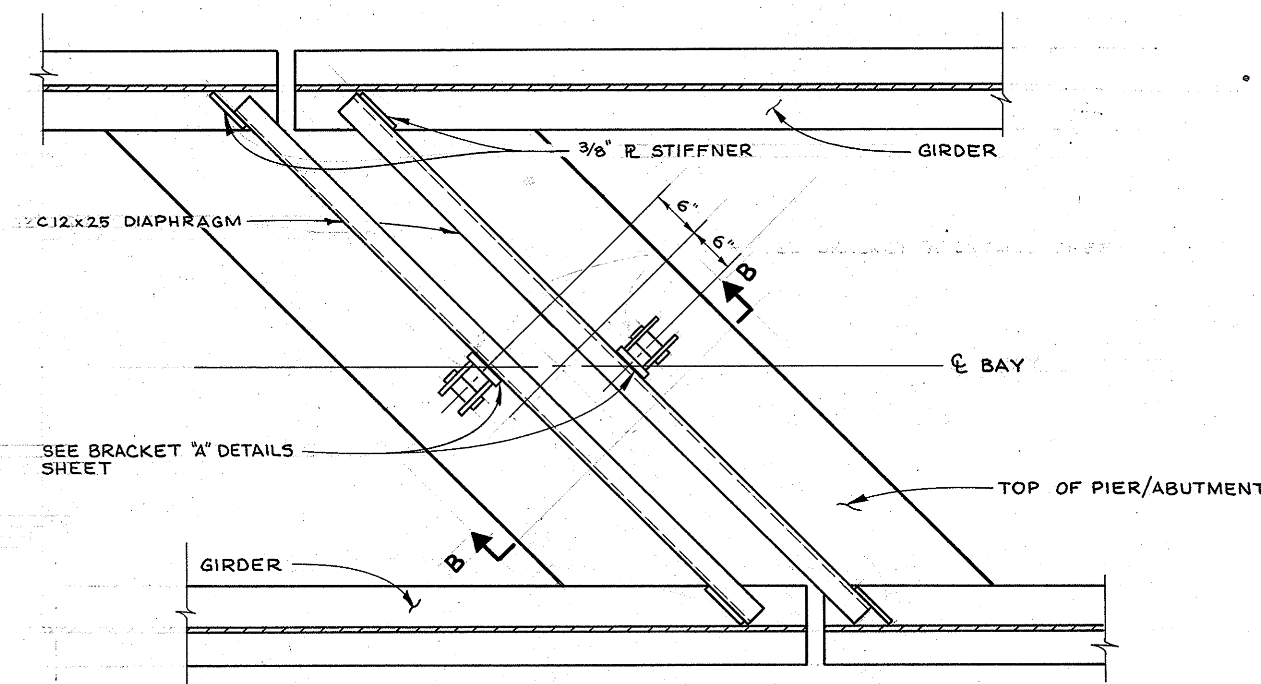
PLAN VIEW NO SCALE
