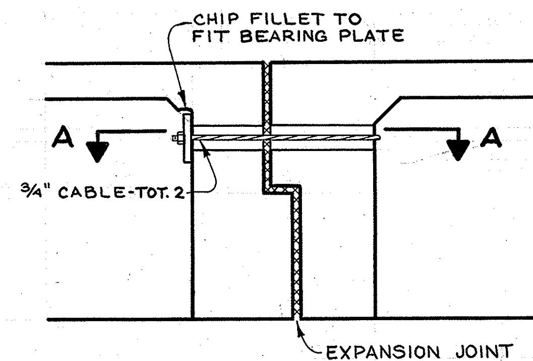
ELEVATION VIEW NO SCALE
