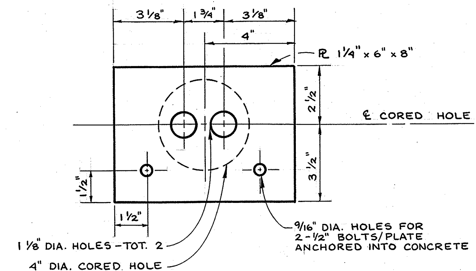
BEARING PLATE DETAIL NO SCALE
