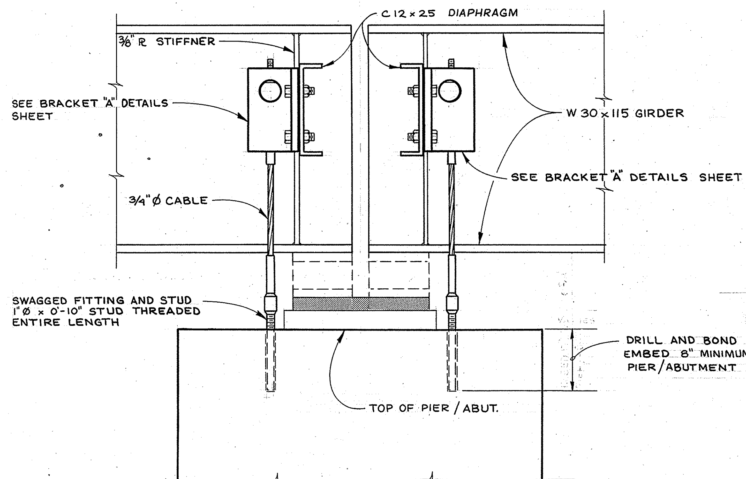
SECTION B-B NO SCALE
