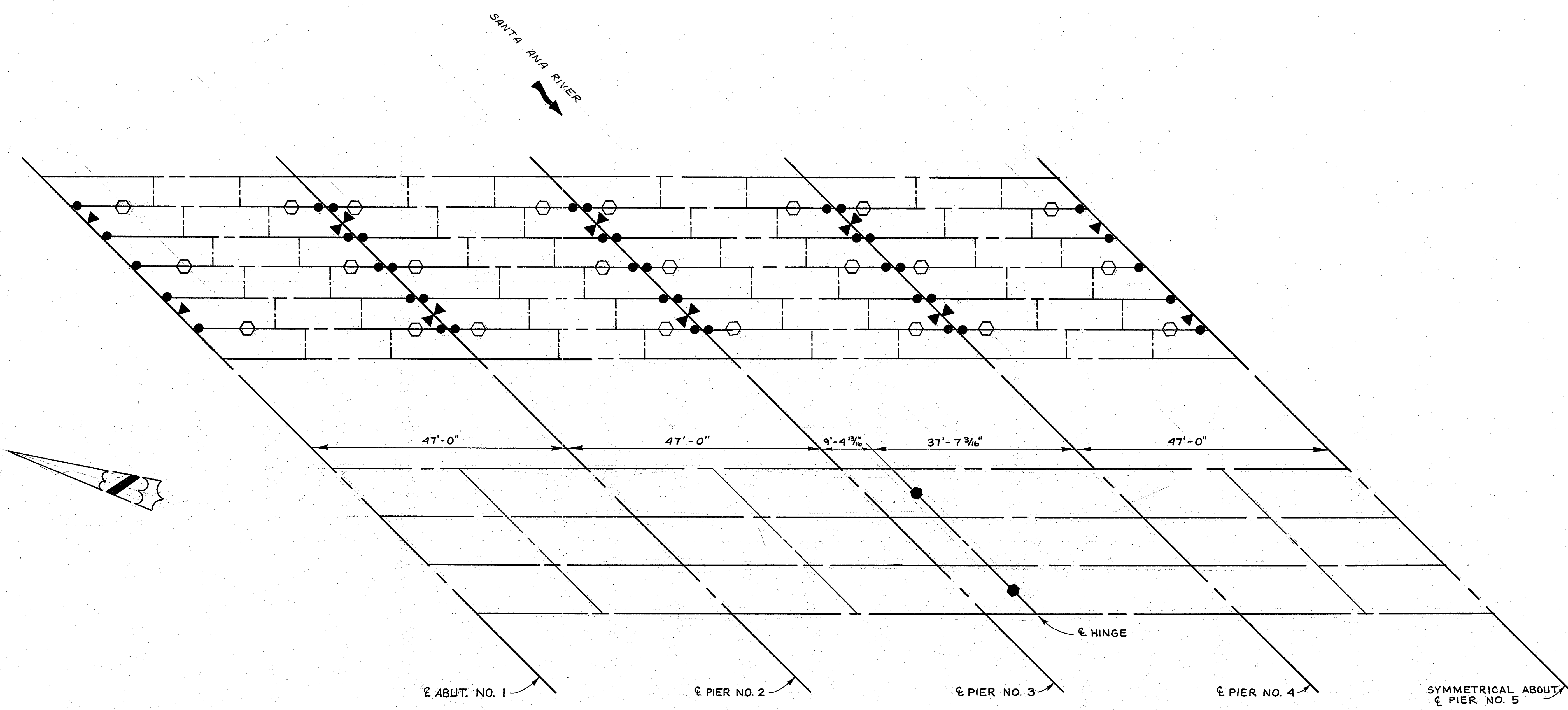
RESTRAINER LAYOUT SCALE 1"=10'
