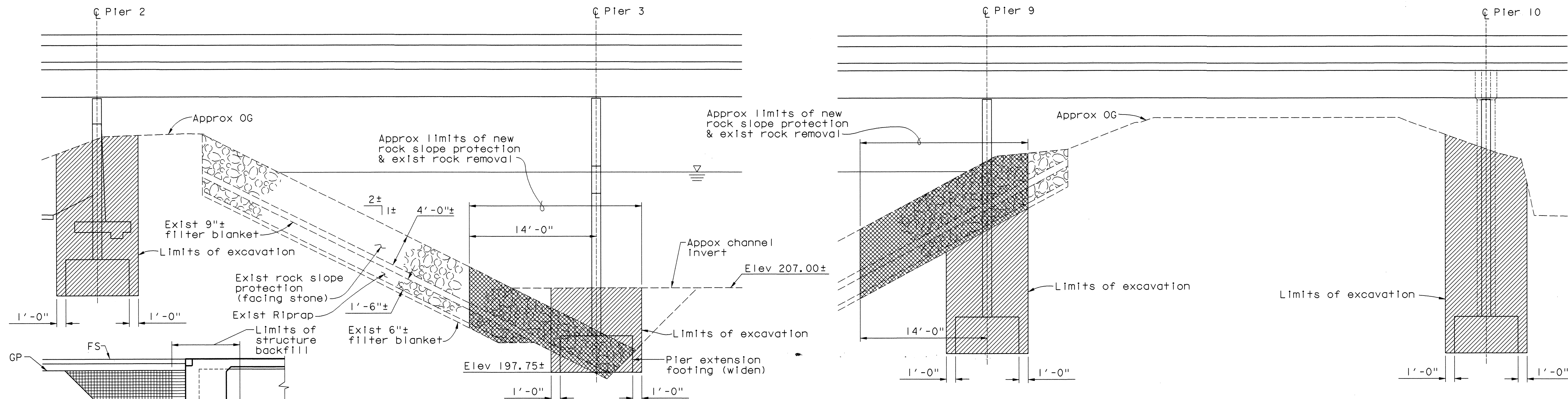
LIMITS OF ROCK SLOPE PROTECTION REPLACEMENT AND EXCAVATION \frac{3}{16}'' = 1'-0''
