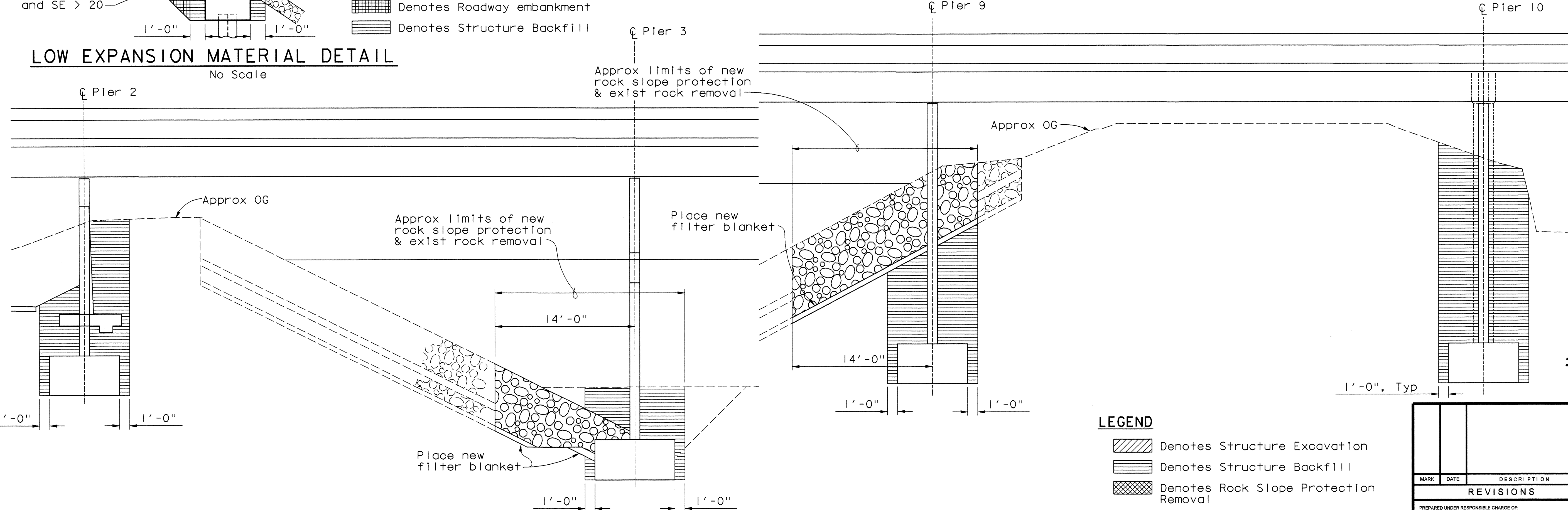
LIMITS OF ROCK SLOPE PROTECTION REPLACEMENT AND EXCAVATION \frac{3}{16}'' = 1'-0''
