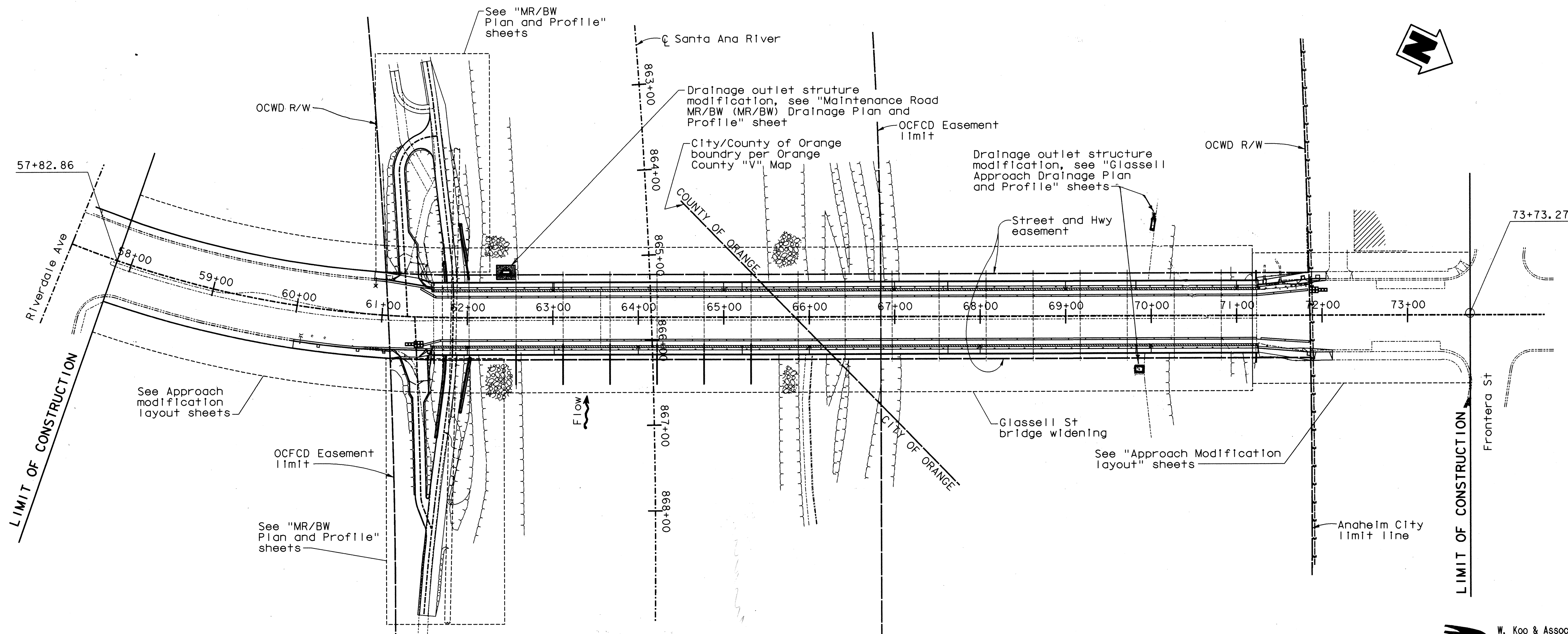
PLAN 1" = 60'
