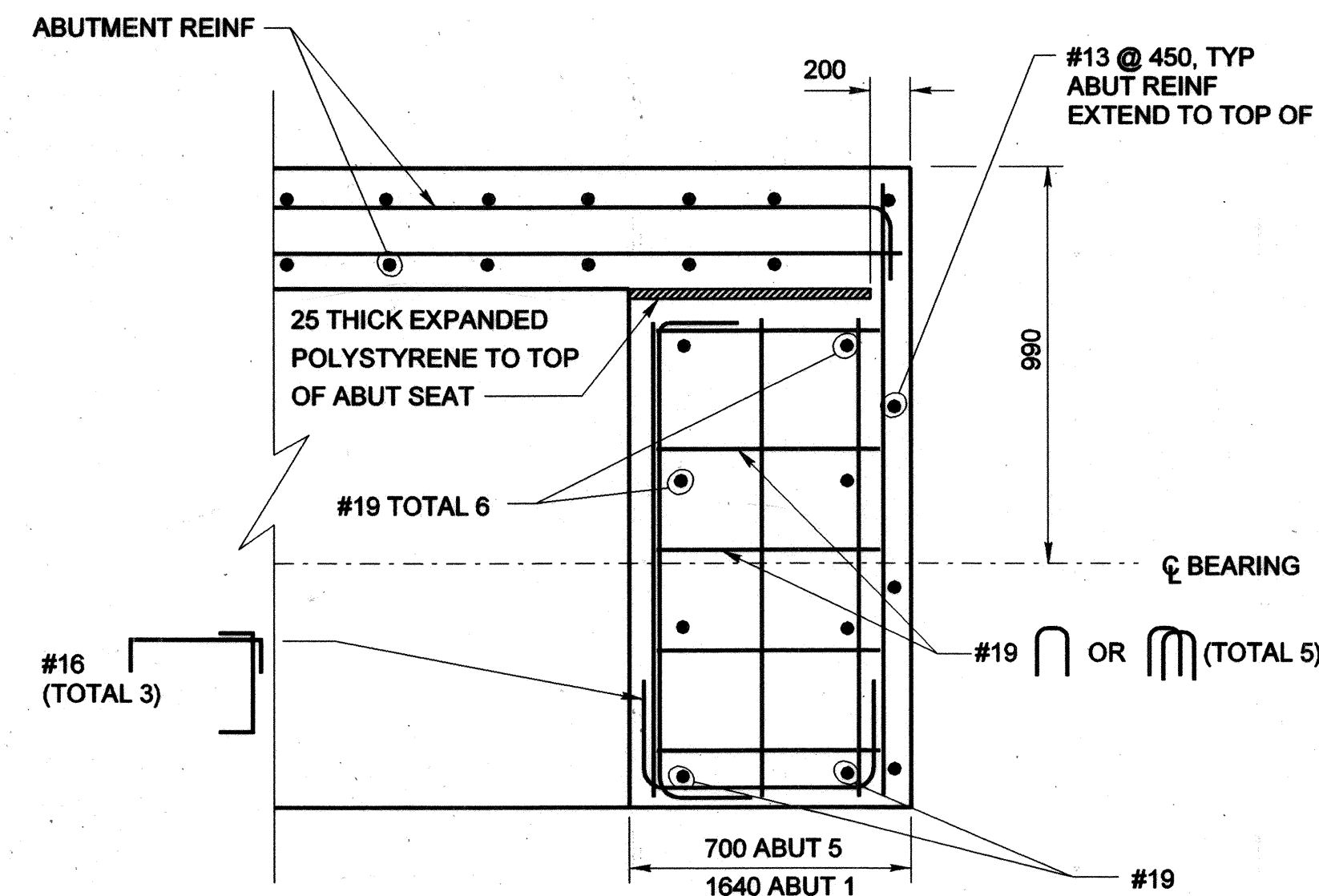
SECTION D - D (ABUTMENT 1 & 5)
