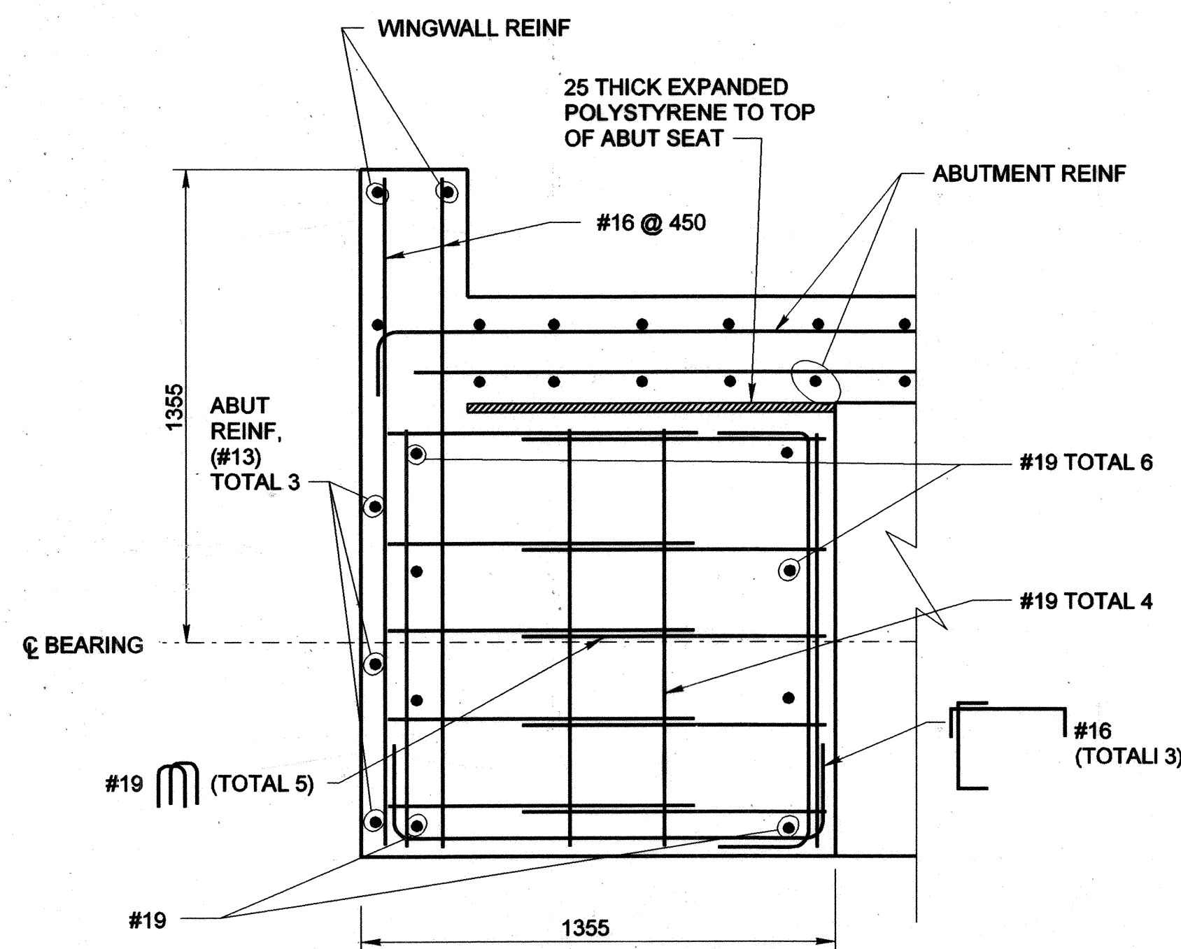
SECTION A - A (ABUTMENT 1 & 5)
