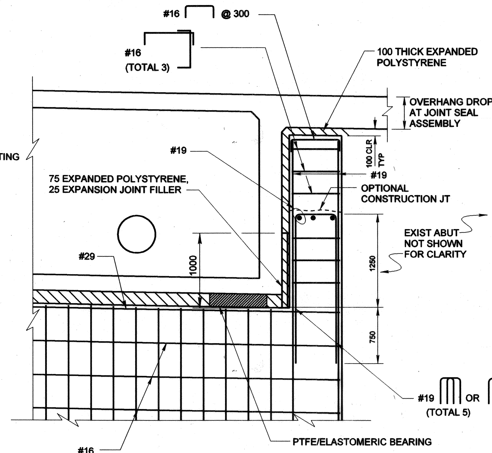
DETAIL SHEAR KEY (ABUTMENT 1 & 5, FOR SECTION D - D)
