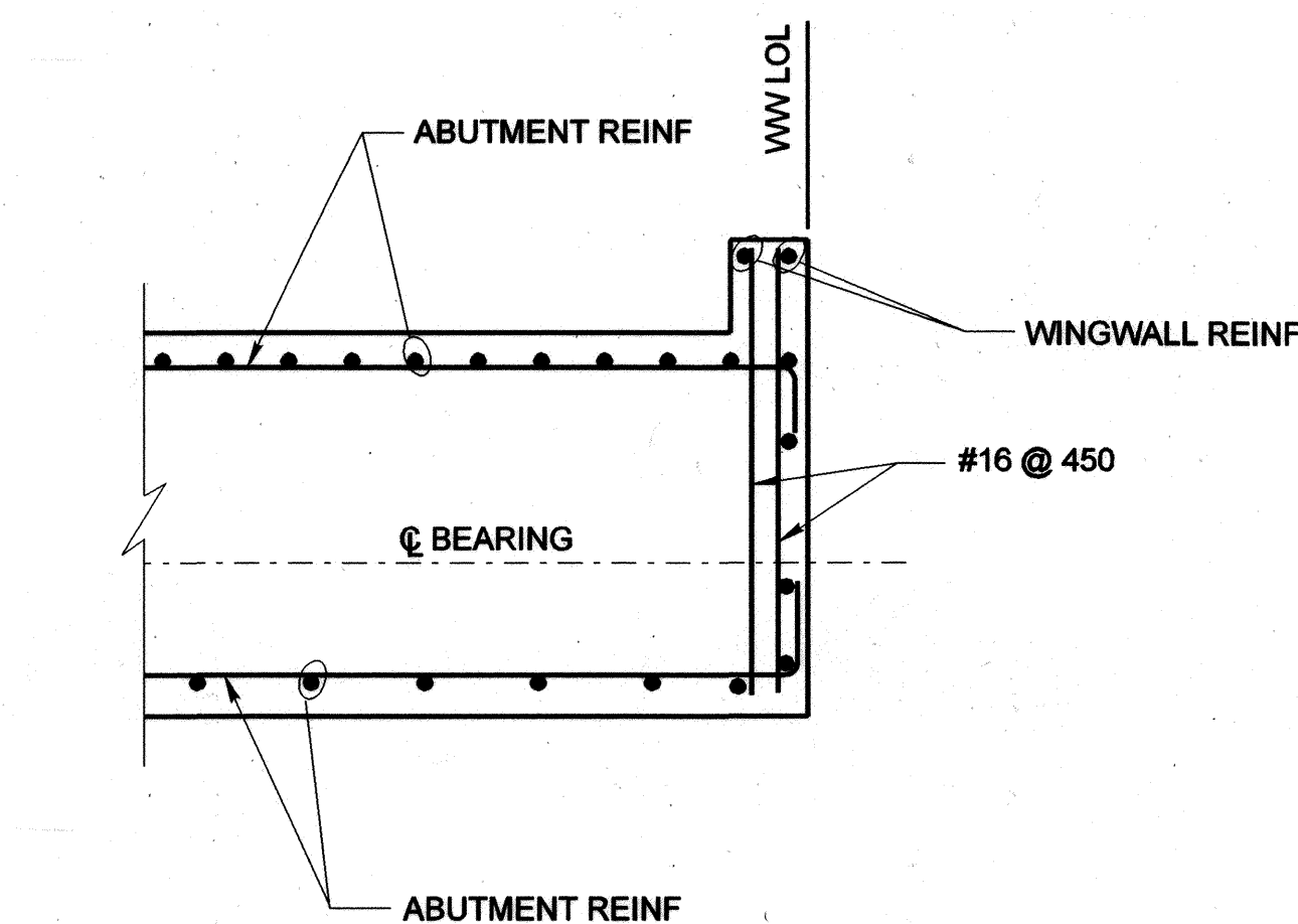
SECTION B - B (TAKEN FROM ABUTMENT DETAILS NO. 1 & 2)
