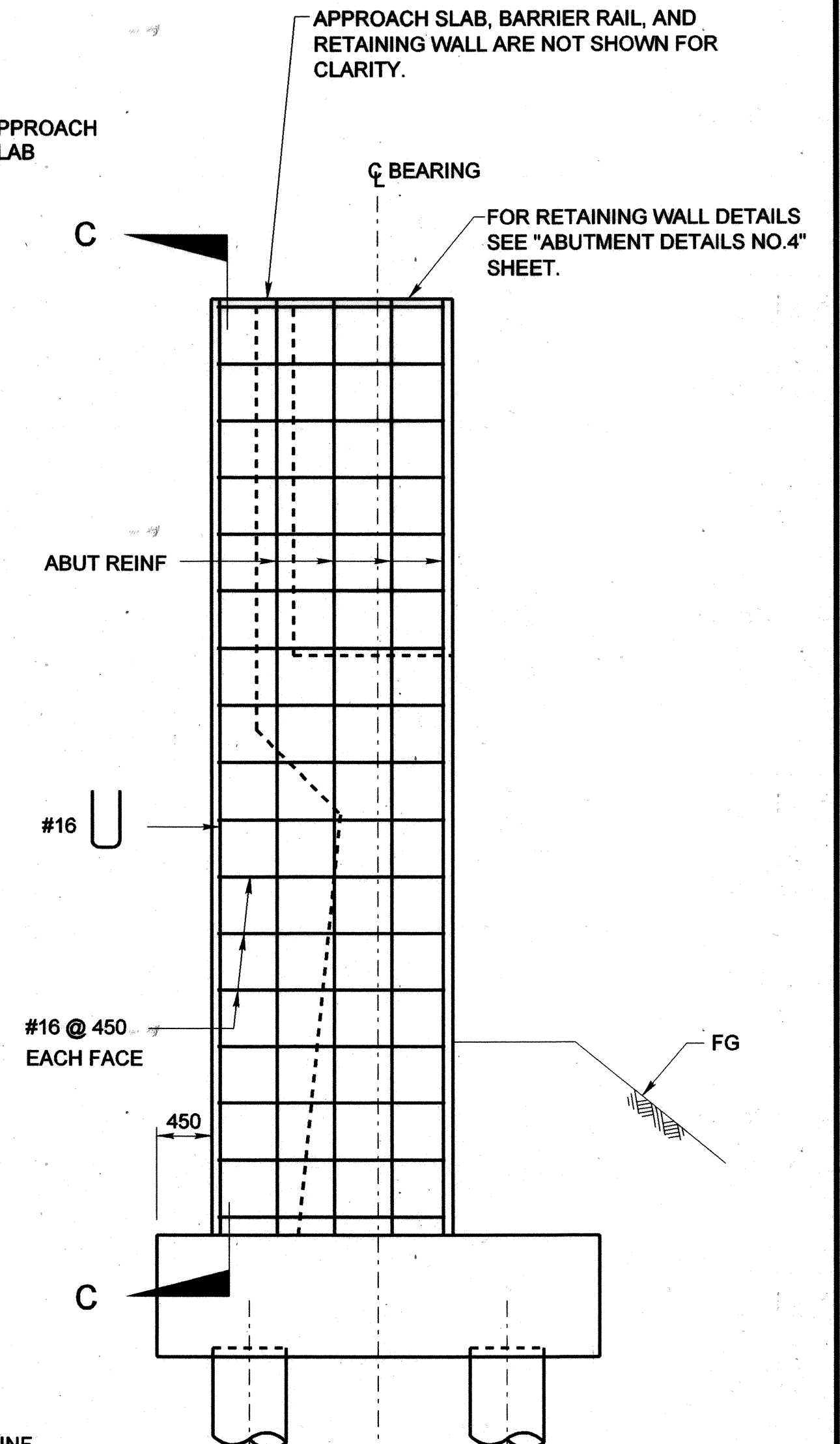
WINGWALL ELEVATION
