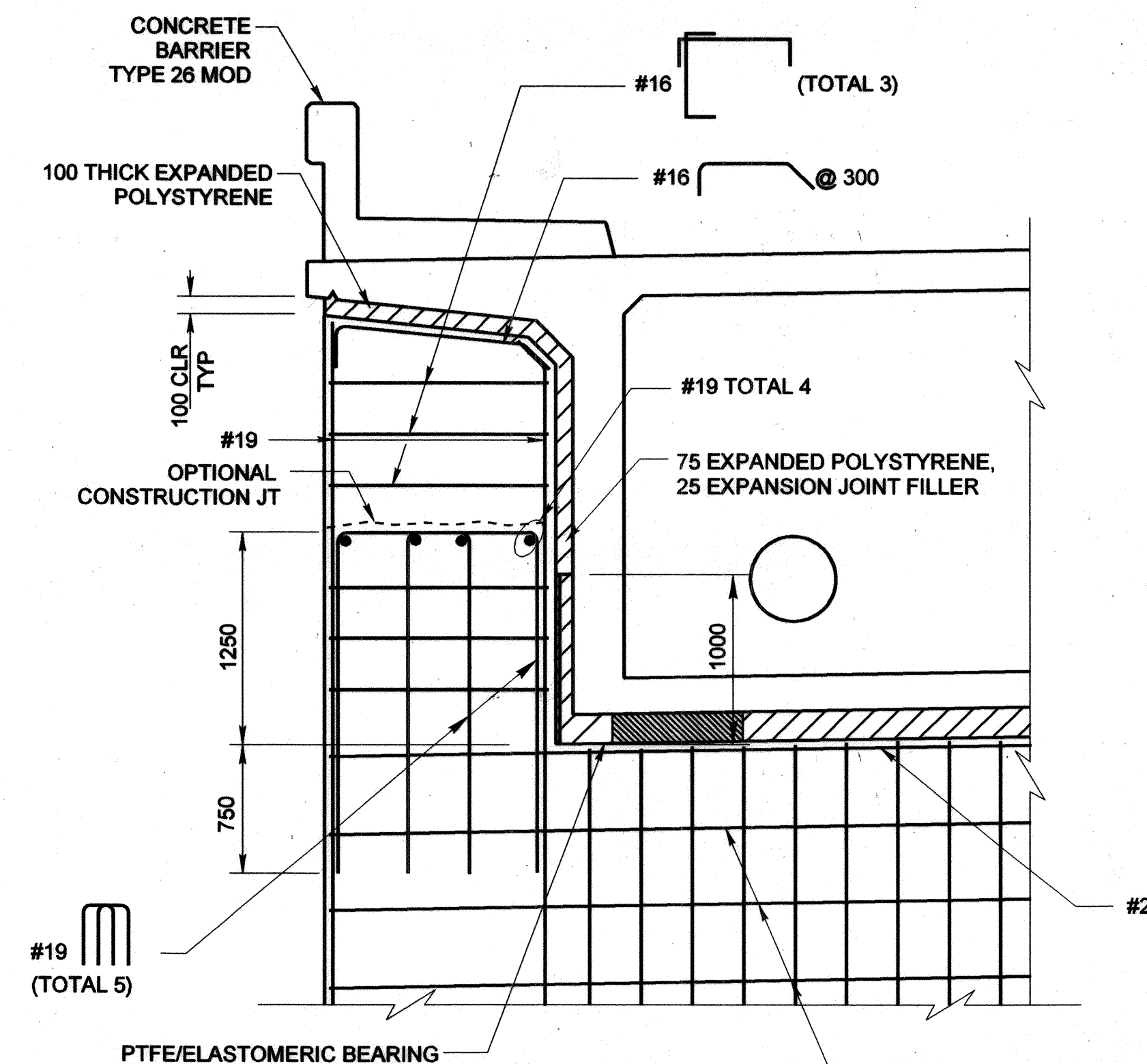
DETAIL SHEAR KEY (ABUTMENT 1 & 5, FOR SECTION A - A)
